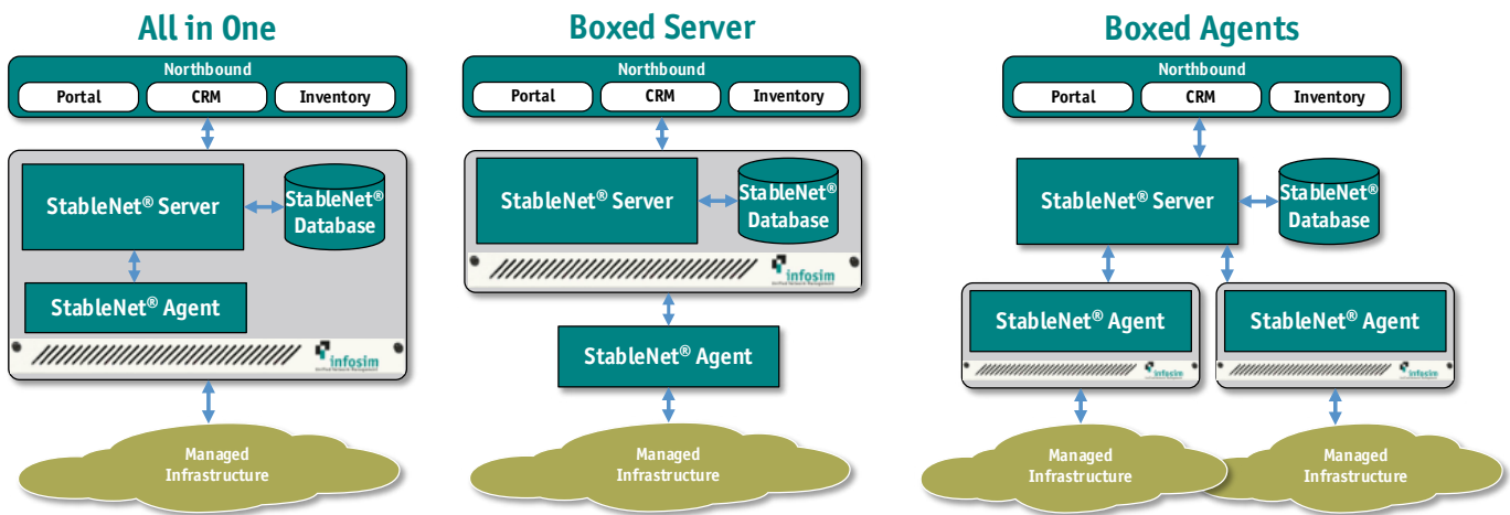
Figure 1: All in One StableNet® Server, StableNet® Database and StableNet® Agent in one box.
